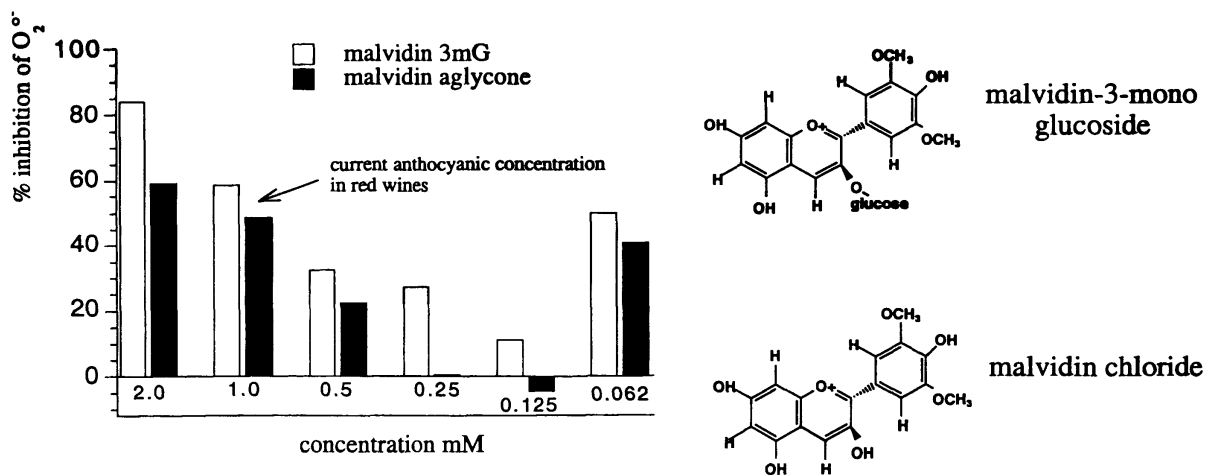
Fig. 3. Comparison between malvidin chloride and malvidin-3-mono-glucoside in aqueous solution.
