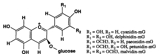
Fig. 1. Structure of grape and wine anthocyanins.
