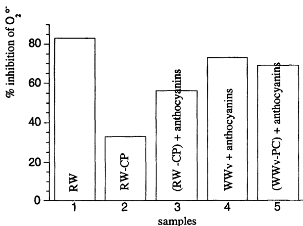
Fig. 4. Free radical scavenging activity (expressed as a percentage of inhibition of O_2^{\bullet -} radicals) of the different samples: 1- RW: 1996 red wine containing 409 mg/l of anthocyanins (measured by discoloration with sodium bisulphite). 2- RW-PC: RW treated with active carbon (loss of all phenolic compounds). 3- (RW-PC) + anthocyanins: (RW-PC) to which 409 mg/l of anthocyanins were added. 4- WWv + anthocyanins: WWv to which 409 mg/l of anthocyanins were added. 5- (WWv-PC) + anthocyanins: (WWv-PC) to which 409 mg/l of anthocyanins were added.
