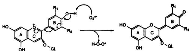
Fig. 2. Diagram of the different hypothetical pathways of oxidation of the anthocyanins by the superoxide O_2^{\cdot-} radical. As the radical is negatively charged, pathway A (attack of the flavylium cation) may be more probable.
